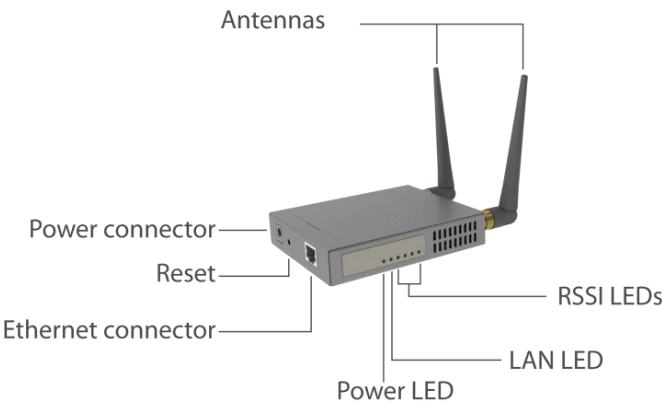
Figure 2 – Vista general del APC 5Mi V2
