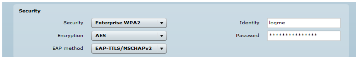
Figure 39 –Wireless Security: Enterprise WPA/WPA2 Security 2
