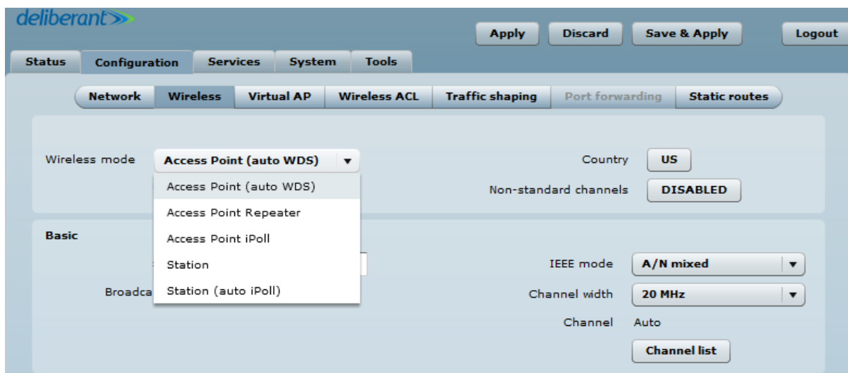
Figure 22 – Device Wireless Operating Mode
